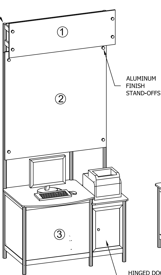
ISOMETRIC (FRONT)
